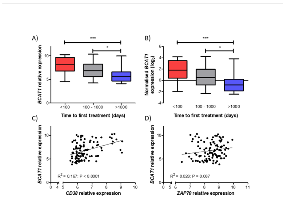
Figure 1 BCAT1 expression levels stratified according to time to first treatment. Microarray data from GEO accession GSE22762; GPL570 platform was stratified according to time to first treatment; <100 days (n=18), 100-1000 days (n=37) and >1000 days (n=40) and analysed for BCAT1 expression (226517_at probe set). The top 100 most dysregulated genes according to this stratification are summarised in Supplemental Table S1. a) Relative BCAT1 expression level at each time point analysed using NCBI GEO2R online tool. b) Normalised BCAT1 expression analysed in GeneSpring (Agilent Technologies) with CG-RMA background correction. c) Linear regression analysis comparing BCAT1 relative expression with CD38 relative expression (205692_s_at probe set). d) Linear regression analysis comparing BCAT1 relative expression with ZAP70 relative expression (214032_at probe set). n=95 for each plot. *P<0.05, ***P<0.001, data analysed by one way-ANOVA with Tukey's Multiple Comparison Test.
