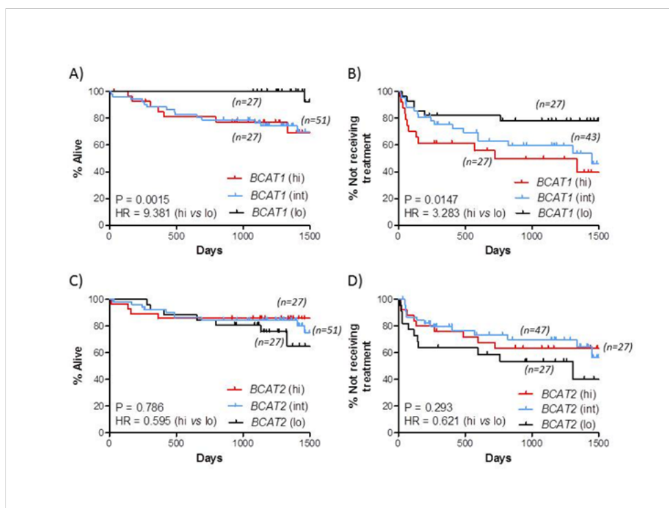
Figure 3 Kaplan-Meier analysis evaluating BCAT1 and BCAT2 expression in CLL. Patients were stratified according to BCAT1 (hi); 2.178 to 4.209 (top quartile) and BCAT1 (lo); -1.187 to -2.686 (bottom quartile), based on averaged \log_2 normalised expression values for each BCAT1 probe set (226517_at; 225285_at; 214452_at and 214390_s_at).
